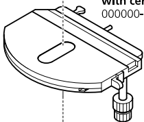
Mechanical stage 75x50/240° R with ceramic coating 000000-1142-561
