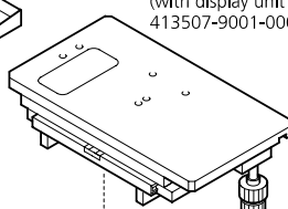
Incident light measuring stage 105x105 R * 000000-1223-326 (with display unit SCD 413507-9001-000)
