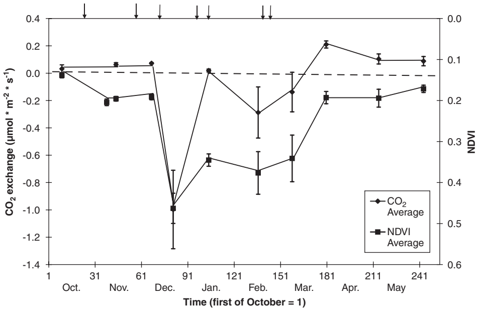
Fig. 3. Seasonal dynamics of the NDVI and the CO 2 exchange for the mixed BSC at the sandy environment at the Agure site. Negative CO 2 exchange mean carbon gain (the arrows indicate the main rain events, more than 5 mm, vertical bars indicate standard deviation n = 21 ).
