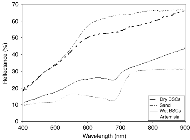
Fig. 1. Spectral reflectances of dry and wet biological soil crusts (BSC), bare sand, and a vascular plant species.
