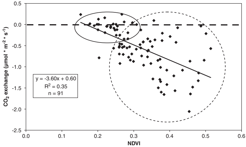
Fig. 7. Correlation between the net CO 2 fluxes of the BSC and the NDVI at the loess environment, for the 2002/3 rainy season. The ellipse and the circle are suggestions to discuss different groups of activity in relation to the basic factor of soil moisture. One, the ellipse, is enclosing data within a group of lower NDVI values corresponding to CO 2 exchange data around zero. The second group (circle) encloses data with increasing NDVI values accompanied by an increase of the CO 2 exchange, which is realized depending on other environmental factors such as light and temperature.
