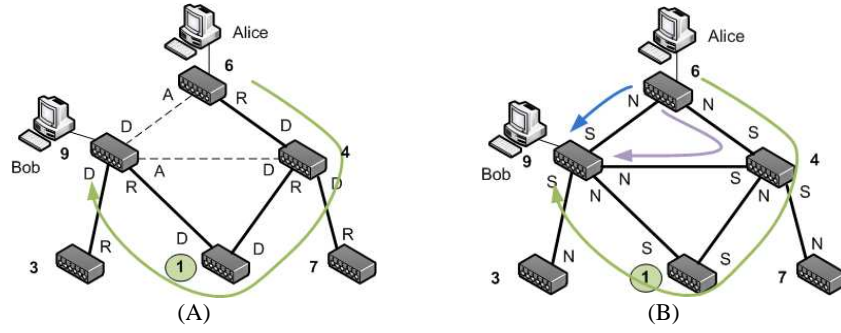
Fig. 2. Forwarding frames from Alice to Bob: (A) Spanning Tree forwarding - unique legal path. (B) Orient forwarding - 3 legal paths.
