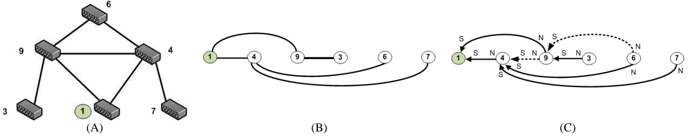
Fig. 1. (A) A communication network example with uniform link and port costs. (B) The result of the spanning tree protocol and its imposed strict total order by root cost paths and bridge IDs. The bridge with the lowest ID, Bridge 1 is the Root bridge. (C) The Orient topology. Dashed edges are edges that do not belong to the spanning tree. North ports are denoted by N and south ports by S . The bridge with the lowest ID, Bridge 1 is the Polaris.
