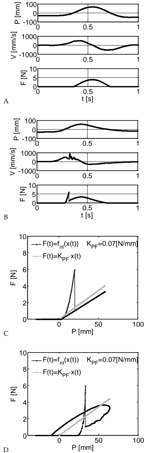
Fig. 6. Example of human-side trajectories from one trial in training phase (A) and two trials in the test phase (B-D). (A-B) Position, velocity, and force as a function of time during interaction with linear elastic force field (A) and nonlinear needle insertion like force field (B). In (B) the sudden drop of forces when "breaking" the rigid boundary caused transient oscillation in the velocity profile, which was suppressed, typically within 100ms. (C-D) Trajectories in force position plane (black) and the linear elastic force field approximation constructed from a regression of position over force information model (gray) in trial without (C) and with (D) delay. Our regression-based model predicts an identical linear force field approximation for both delayed and non-delayed nonlinear force field. (C) is a re-plot of (B) in a force position plane.
