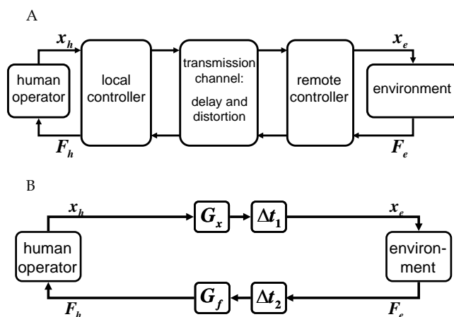
Fig. 1. Teleoperation system: (A) In the general case the human operator (a surgeon) acts through a local controller, a channel, and a remote controller on the remote environment with delayed and distorted feedback. (B) In a simplified case, the human operator interacts with a haptic environment that simulates an architecture that includes only delay ( \Delta t ), transmission gain ( G ), and nonlinear tissue-like environment. x_h and F_h are the position of the human operator's hand and the forces applied on it by the local robotic device (haptic interface) respectively, and x_e and F_e are the simulated position of the remote device and the force exerted by the environment on the device.
