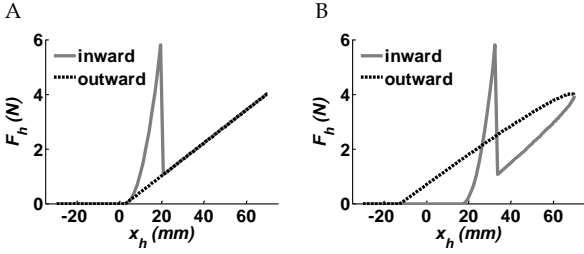
Fig. 2. A nonlinear force field approximates the force profile during needle insertion. (A) Trajectory of nonlinear tissue force field in force-position space. The operator first encounters a rigid nonlinear boundary on the way into the force field, and only after a penetration of 17mm, there is a sudden drop in the applied forces. From that point, the force field is equivalent to a linear one-sided spring. (B) Trajectory of nonlinear tissue force field with delay: force lags position, and therefore, a hysteresis-like trajectory is formed.
