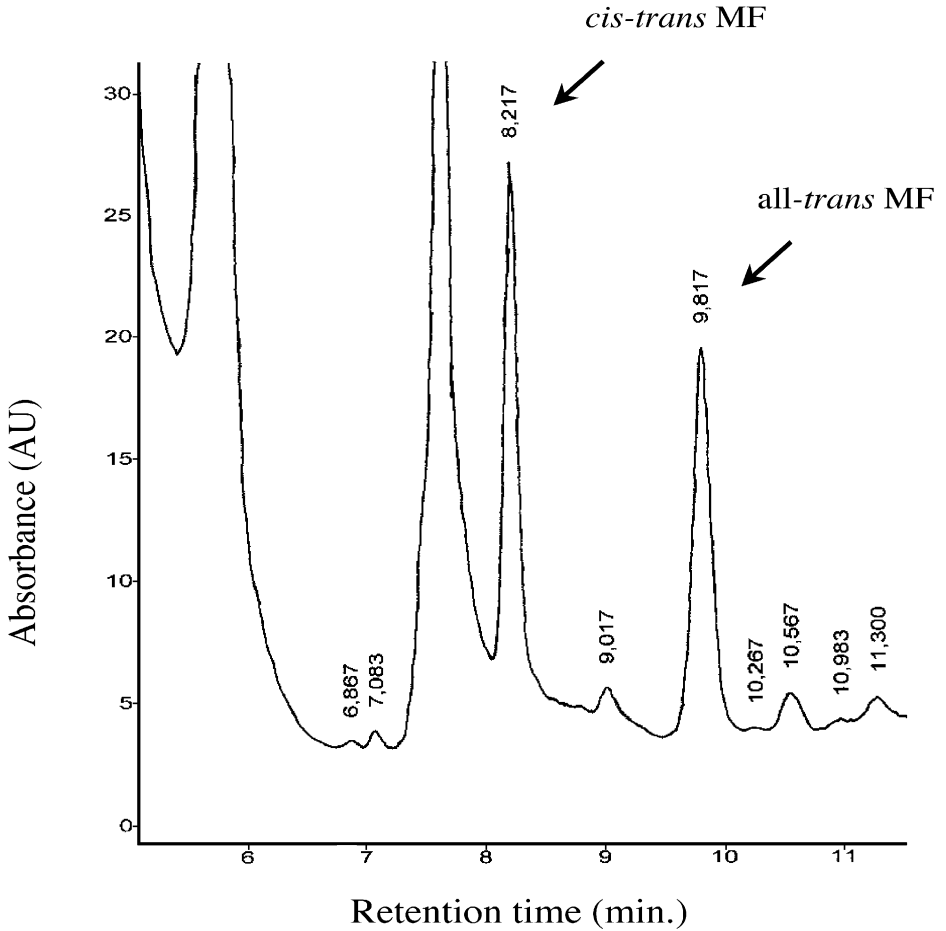
Fig. 1. A representative HPLC chromatogram showing trans-trans MF, the biological isomer, in the hemolymph of a C. quadricarinatus female. cis-trans MF, the nonbiological isomer, served as the internal standard.
