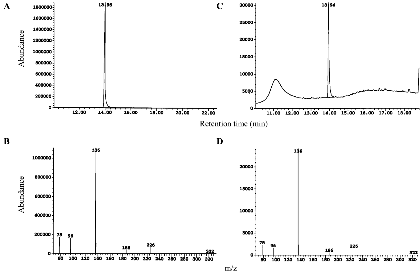
Fig. 3. Representative GC/MS confirming the presence of pyriproxyfen in treated C. quadricarinatus females. (A) GC-MS chromatogram of spiked pyriproxyfen std. serving as reference standard; (B) MS fragmentation of the peak in chromatogram A; (C) GC-MS chromatogram of pyriproxyfen, post treatment, isolated from the hepatopancreas of a treated female; (D) MS fragmentation of the peak in chromatogram C.
