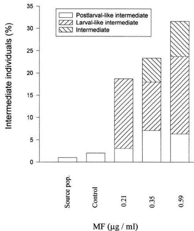
Figure 7. Relative abundance of Macrobrachium rosenbergii intermediate types in experimental groups exposed to different doses of methyl farnesoate, in an untreated control group and a sample from a normal hatchery population.
