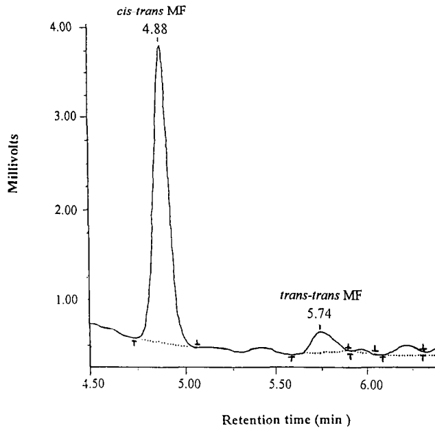
Figure 1. HPLC detection of methyl farnesoate in Macrobrachium rosenbergii larvae at stage 4. Cis-trans methyl farnesoate was used as the internal standard.
