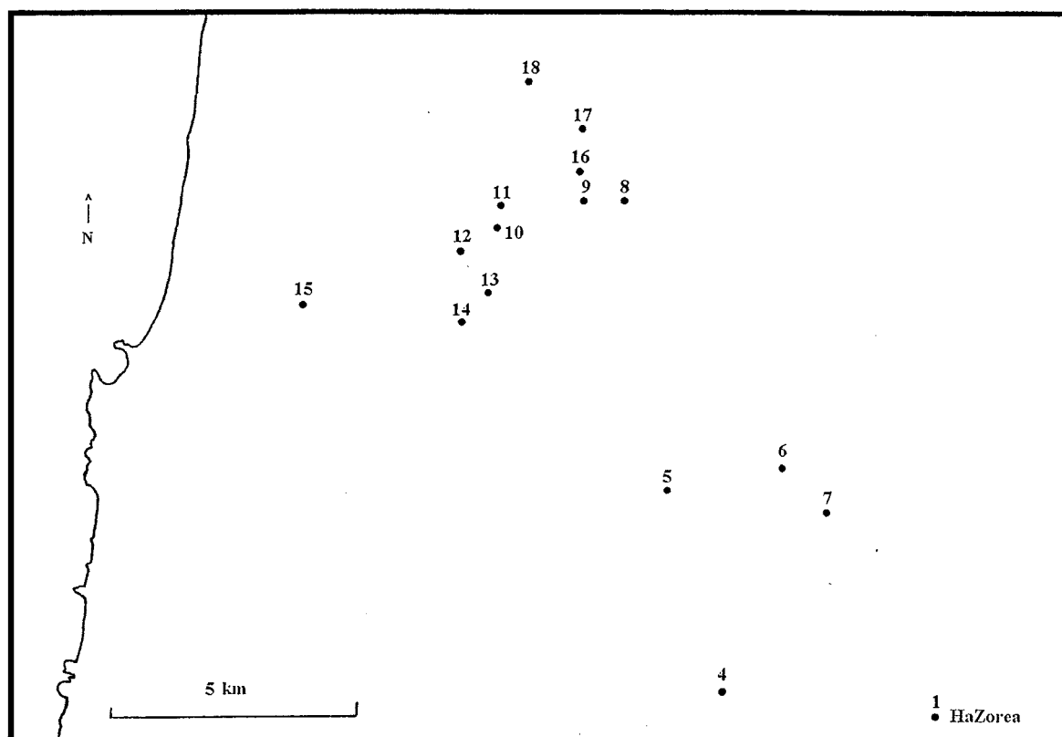
FIG. 2. Biomonitoring sites in the Carmel mountain region. 1, HaZorea Forest; 4, Mevo Elyakim; 5, Oren HaSela parking site; 6, Keren HaCarmel road junction; 7, Keren HaCarmel; 8, Oranei HaPisgah; 9, Damun Junction; 10, Beit Oren; 11, Kedumim quarry; 12, artificial lake; 13, Rakit; 14, Yearoth HaCarmel Hotel; 15, Nahal Oren mouth; 16, Carmel Park office; 17, antenna; 18, Hai Bar.
