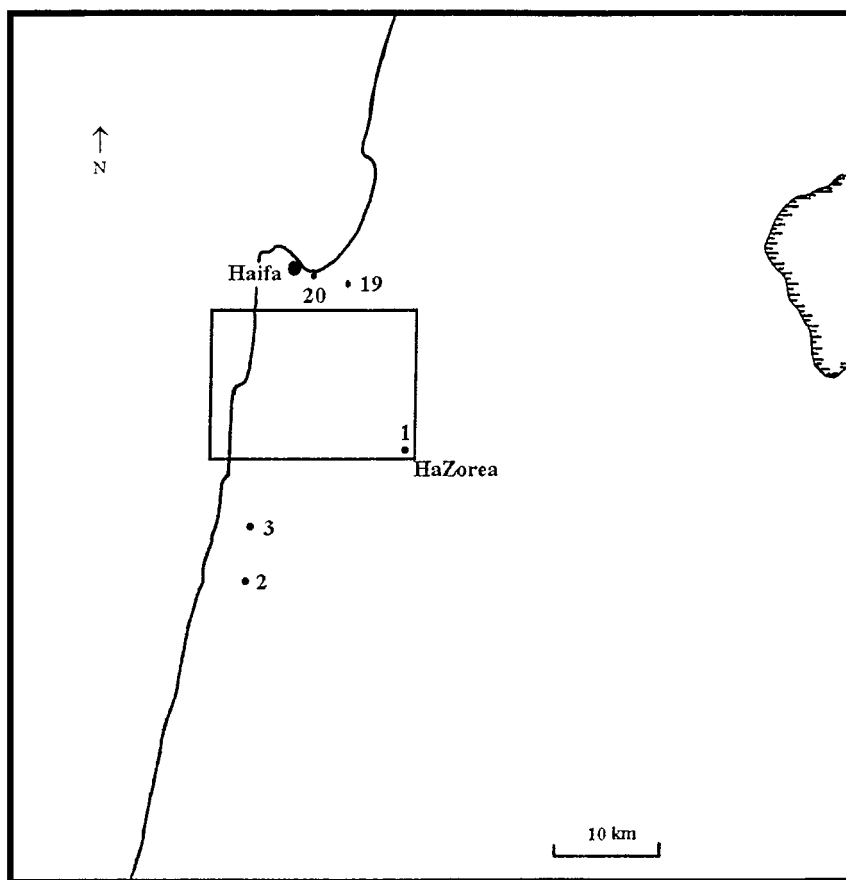
FIG. 1. The northern part of Israel, indicating HaZorea, the Haifa Bay (sites 19 and 20), site 2 (Jabotinski Park), and site 3 (Ramat HaNadiv).
