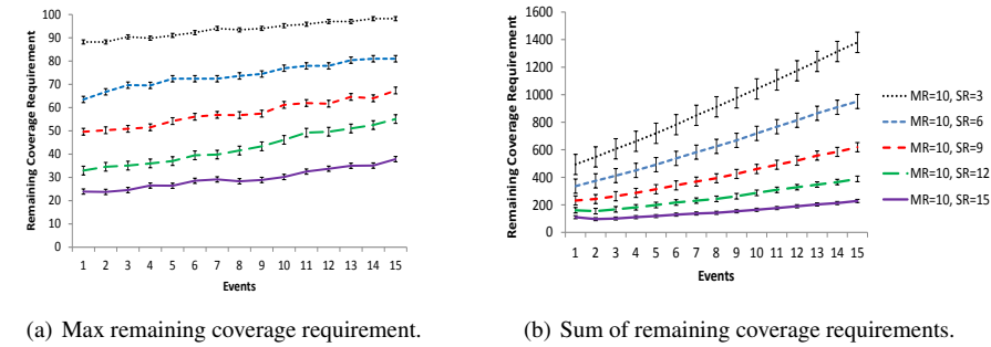
Fig. 14 Effect of varying sensing range on MGM_MST with submodular joint credibility function F_{cprob} .
