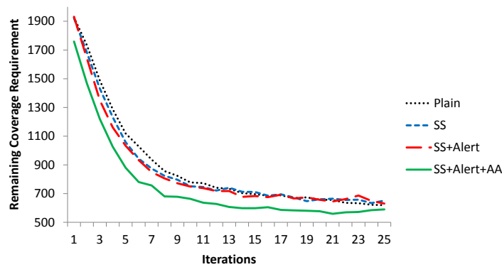
Fig. 26 Sum of remaining coverage requirements for different levels of cooperation.
