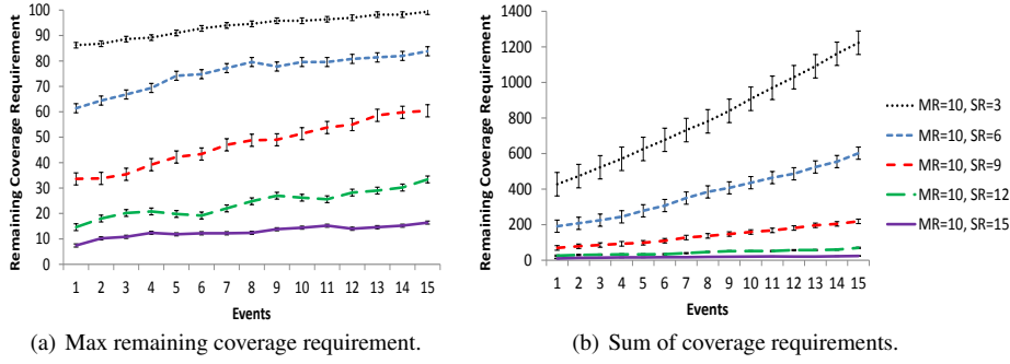
Fig. 12 Effect of varying sensing range on MGM_MST with additive joint credibility function F_{sum}^3 .
