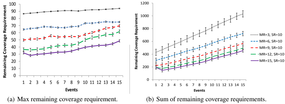
Fig. 13 Effect of varying mobility range on MGM_MST with submodular joint credibility function F_{cprob} .
