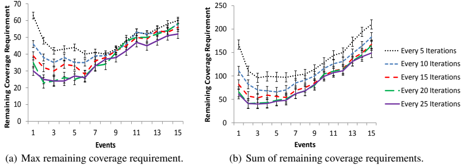
Fig. 22 Effect of varying period of DSA_PILR.
